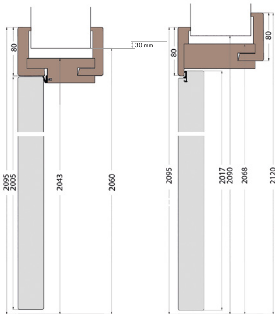
Standard swing system
