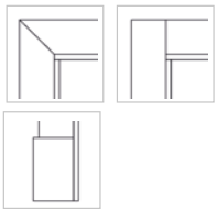
7. Adjustable doorframe with bottom plinths
