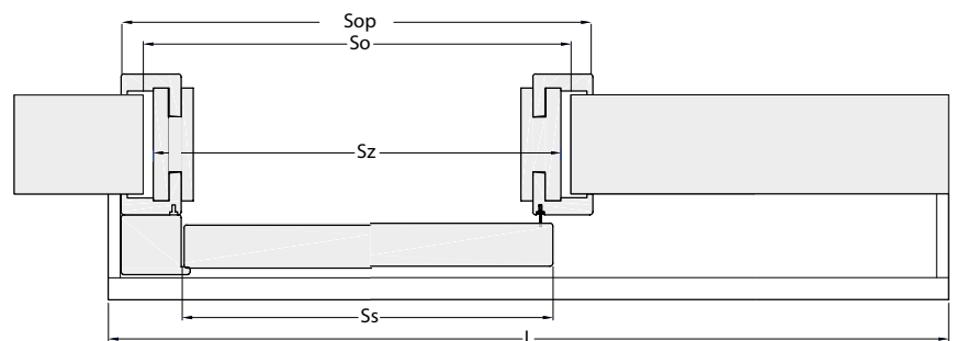
Single Wall-Mounted Sliding System
